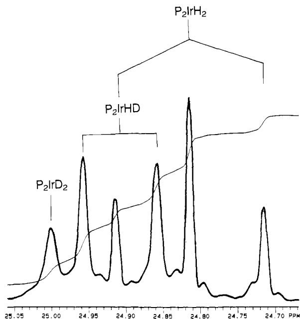
Figure 1. 161.9-MHz ^{31}\text{P} NMR spectrum of a \text{dmf-}d_7 solution of [(\text{Ph}_3\text{P})_2\text{IrH}_2]_3\text{PW}_{12}\text{O}_{40} after exchange with \text{D}_2 showing (\text{Ph}_3\text{P})_2\text{IrH}_2(\text{dmf})_2^+ , (\text{Ph}_3\text{P})_2\text{Ir}(\text{HD})_2(\text{dmf})_2^+ , and (\text{Ph}_3\text{P})_2\text{IrD}_2(\text{dmf})_2^+ .
