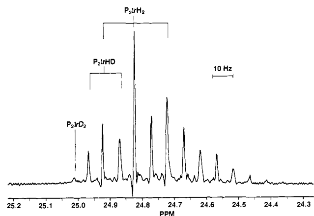
Figure 4. Resolution-enhanced ^{31}\text{P} NMR spectrum of rearranged [(\text{Ph}_3\text{P})_2\text{Ir}(\text{H},\text{D})_2]_3\text{PW}_{12}\text{O}_{40} ( \text{dmf}-d_7 solvent).
