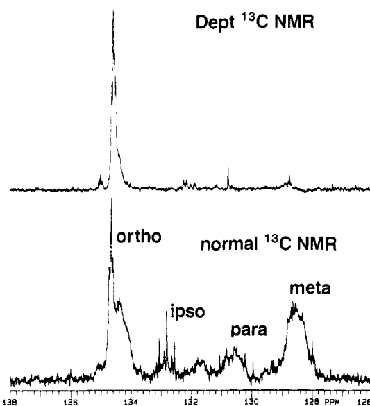
Figure 2. DEPT ^{13}\text{C} NMR spectrum of rearranged [(\text{Ph}_3\text{P-}d_{15})_2\text{IrH}_2]_3\text{PW}_{12}\text{O}_{40} in \text{dmf-}d_7 .
