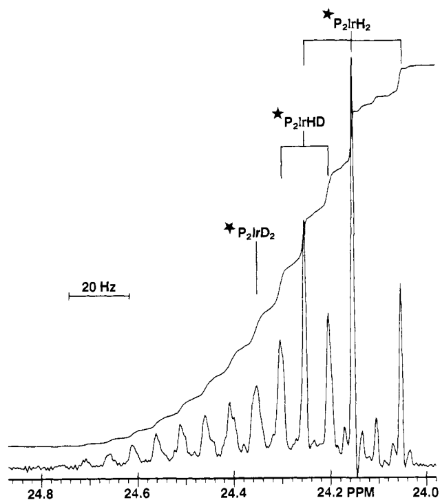
Figure 3. Resolution enhanced 161.9-MHz ^{31}\text{P} NMR spectrum, with single frequency decoupling of the aromatic protons, of rearranged [(\text{Ph}_3\text{P}-d_6)_2\text{IrH}_2]_3\text{PW}_{12}\text{O}_{40} in \text{dmf}-d_7 . *P indicates \text{Ph}_3\text{P}-d_6 .
