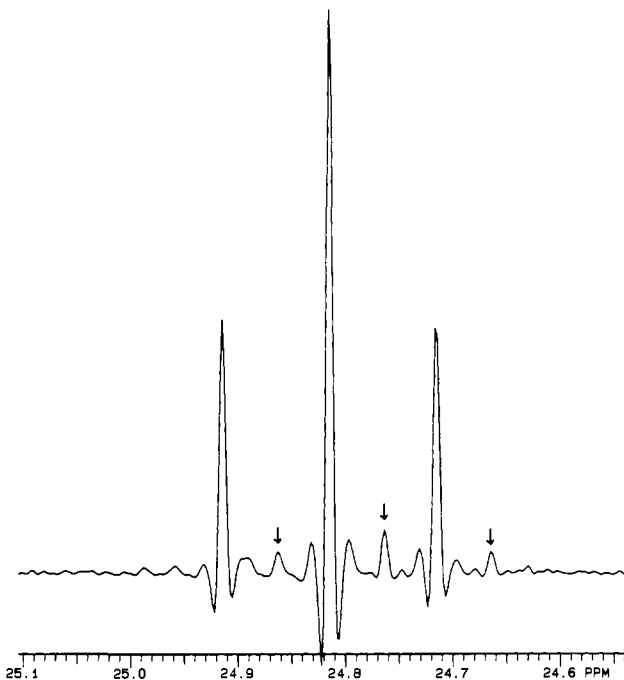
Figure 5. Resolution enhanced 161.9-MHz ^{31}\text{P} NMR spectrum of [(\text{Ph}_3\text{P})_2\text{IrH}_2]_3\text{PW}_{12}\text{O}_{40} after reaction with \text{C}_6\text{D}_{12} ( \text{dmf}-d_7 solvent). Arrows indicate the 1:2:1 triplet due to (\text{Ph}_3\text{P})(\text{Ph}_3\text{P}-d_1)\text{IrH}_2(\text{dmf})_2^+ .
